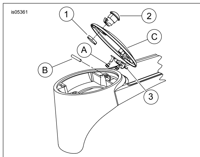
Figure 1. Service Parts: Console Pushbutton Fuel Door Release
