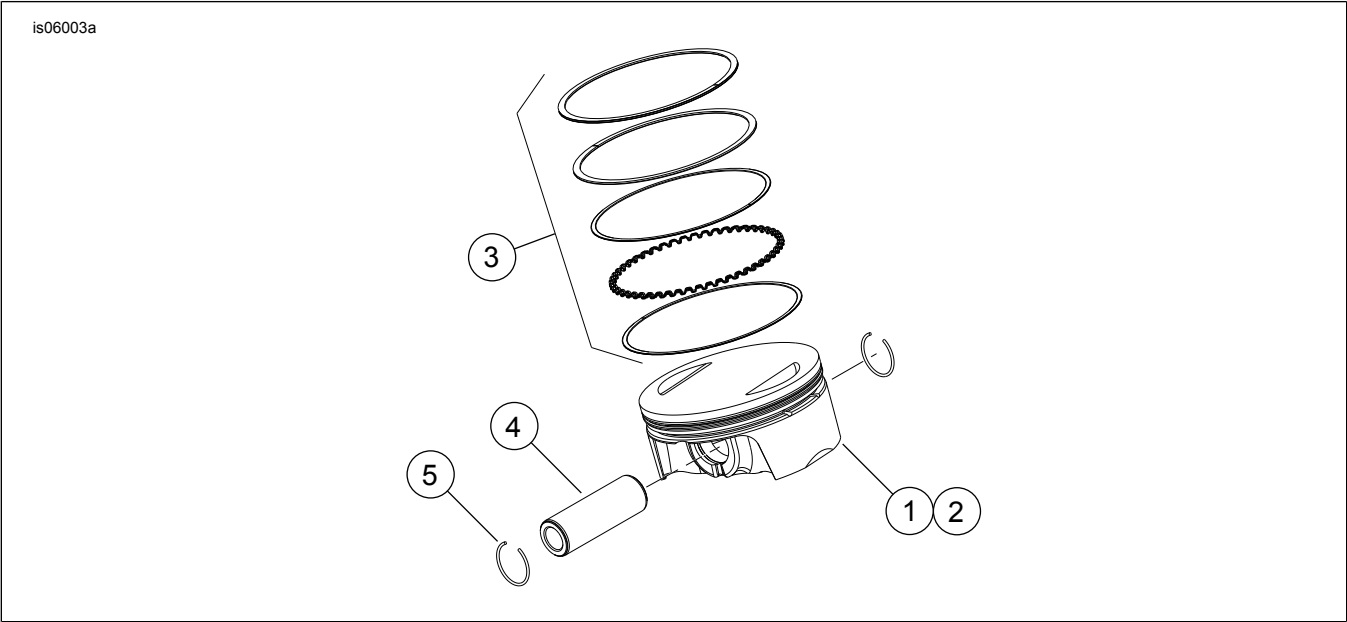
Figure 3. Service Parts: Screamin' Eagle Pro Twin Cam Stroker Piston Kits for Stock Cylinder Heads
