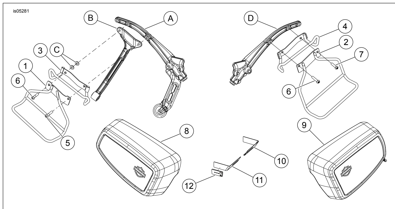
Figure 5. Service Parts: XR1200 Saddlebags
