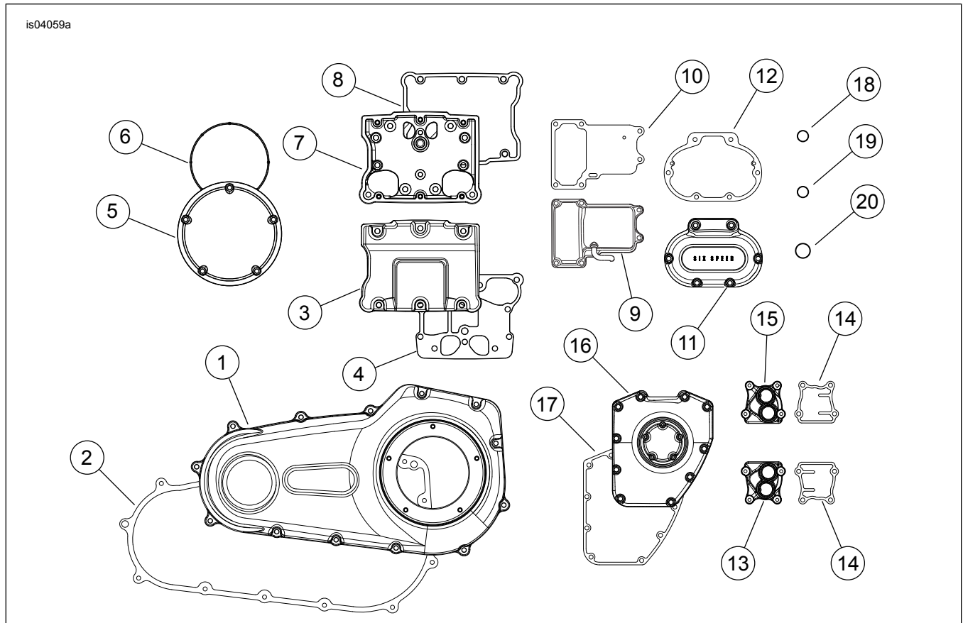
Figure 1. Service Parts, Chrome Engine Cover Kit
