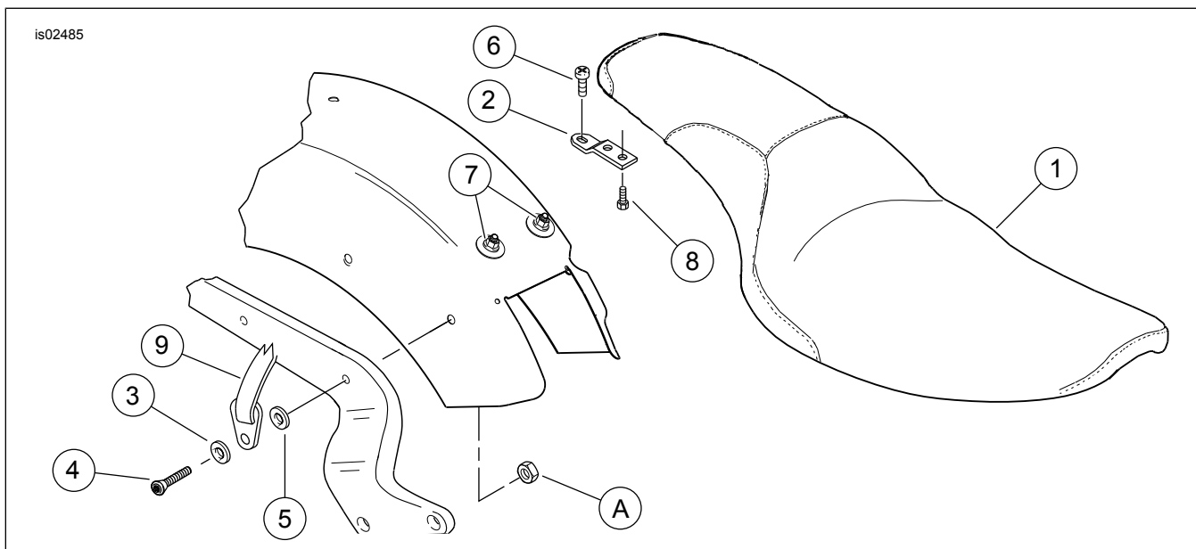
Figure 3. Service Parts: Softail Seat Kit
