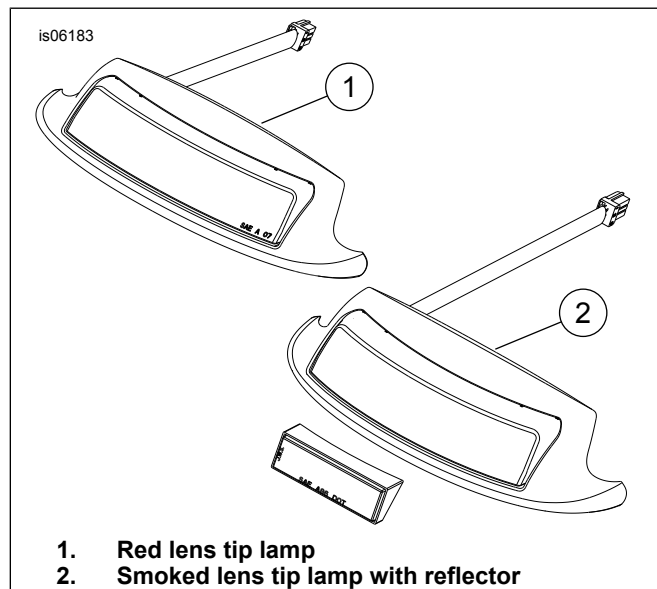
Figure 1. Fender Tip Lamps, Run and Brake
