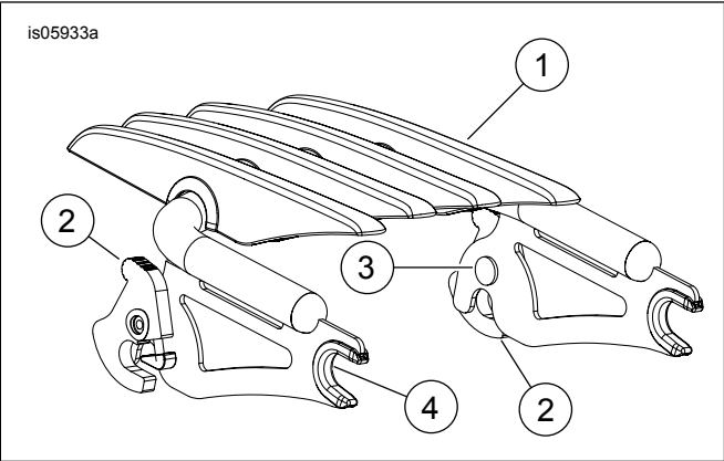
Figure 3. Service Parts: H-D Detachables Stealth Luggage Rack
