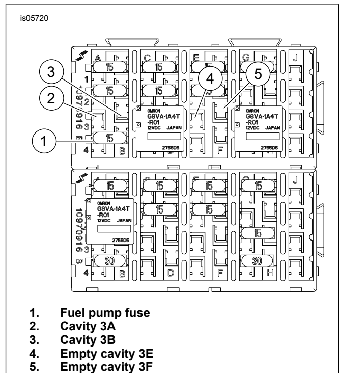
Figure 4. Fuse Block (2008-Earlier Models Shown)
