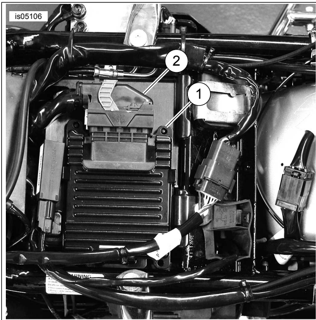
Figure 1. Electronic Control Module (ECM)
