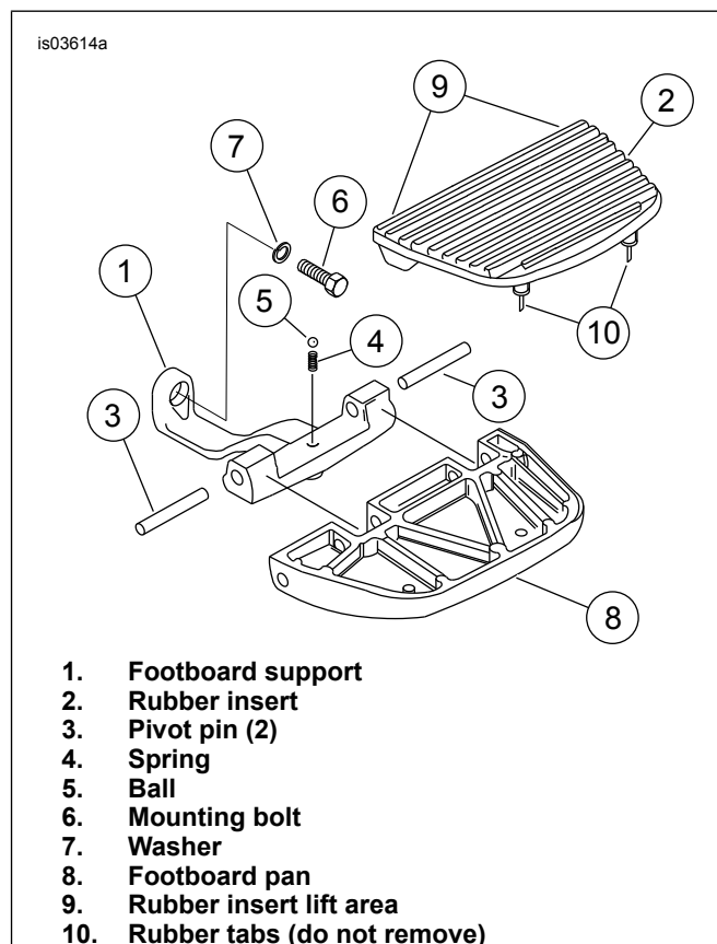
Figure 1. Stock Footboard Mounting
