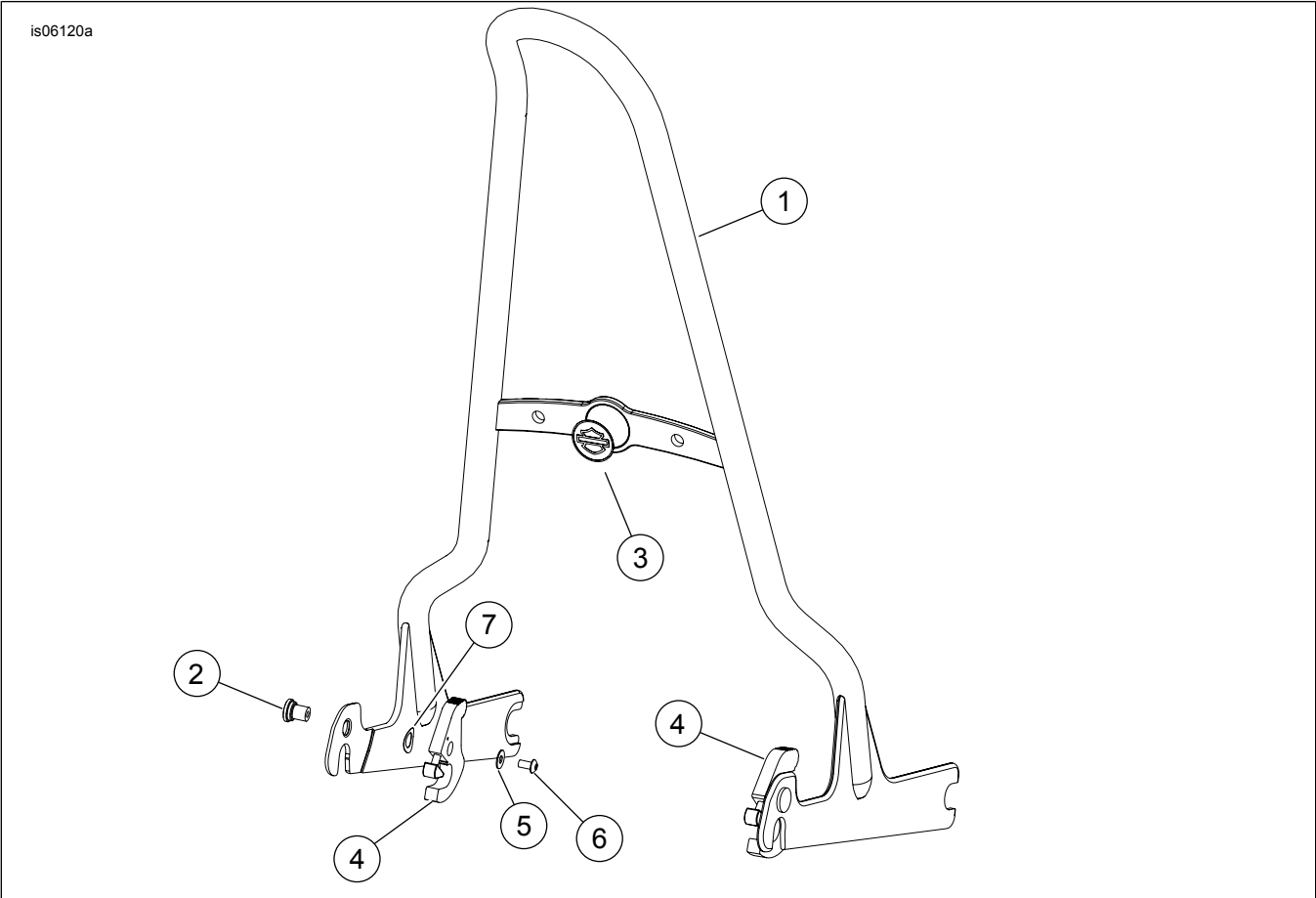
Figure 3. Service Parts: H-D Detachables Upright
