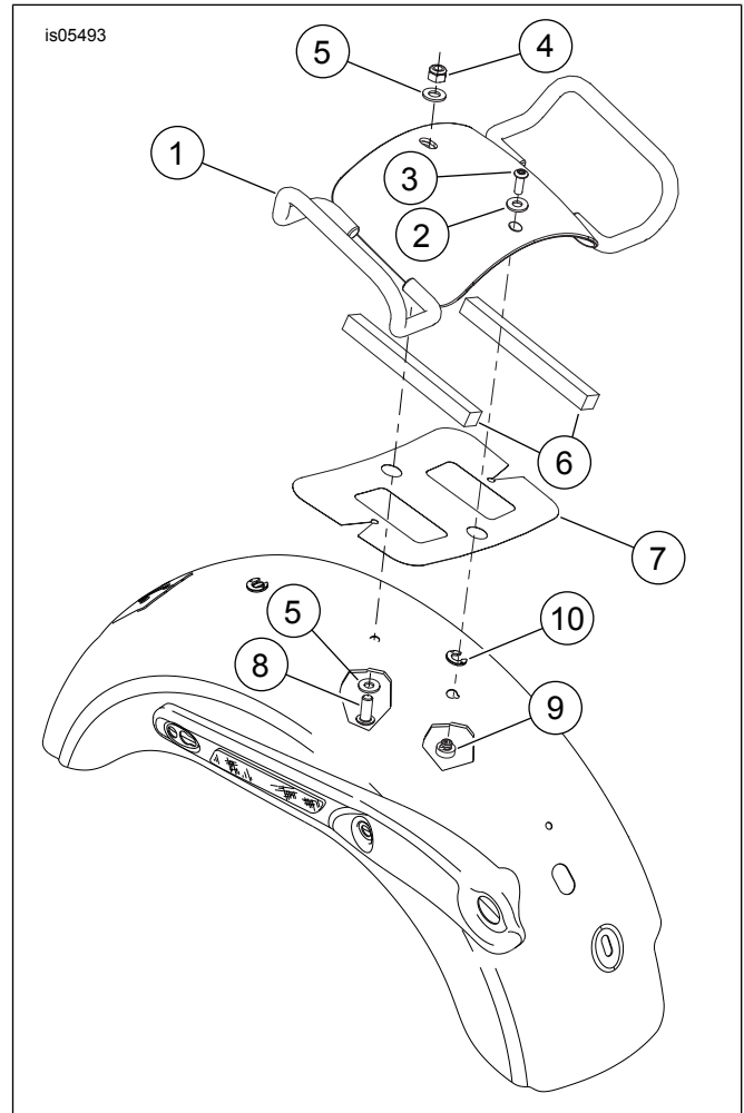
Figure 1. Service Parts: Passenger Grab Rail
