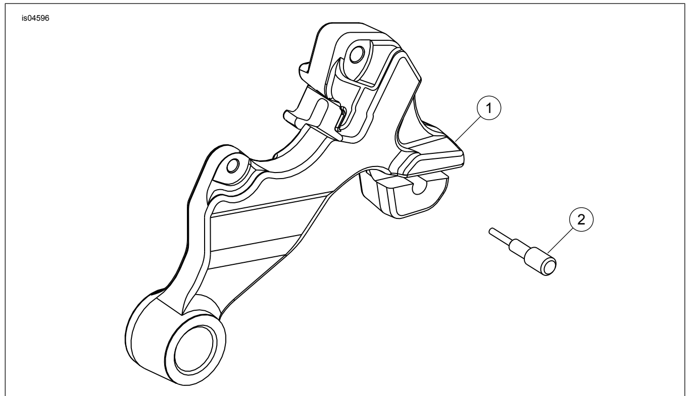
Figure 1. Service Parts: Rear Caliper Bracket Assembly
