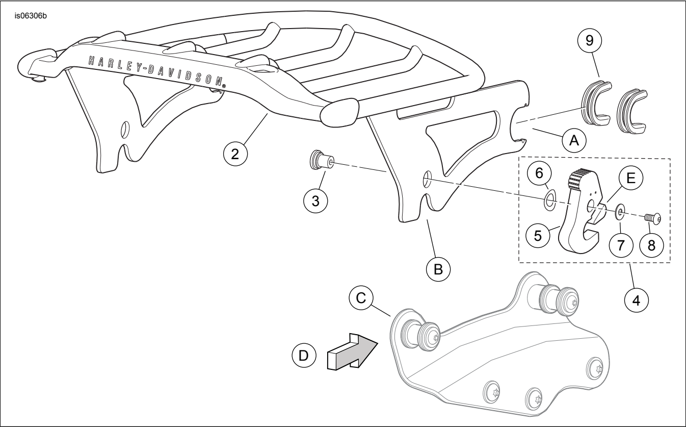
Figure 3. Service Parts, H-D Detachables Air Wing Two-Up Luggage Rack
