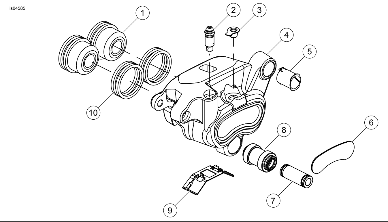
Figure 1. Service Parts: Rear Caliper Assembly
