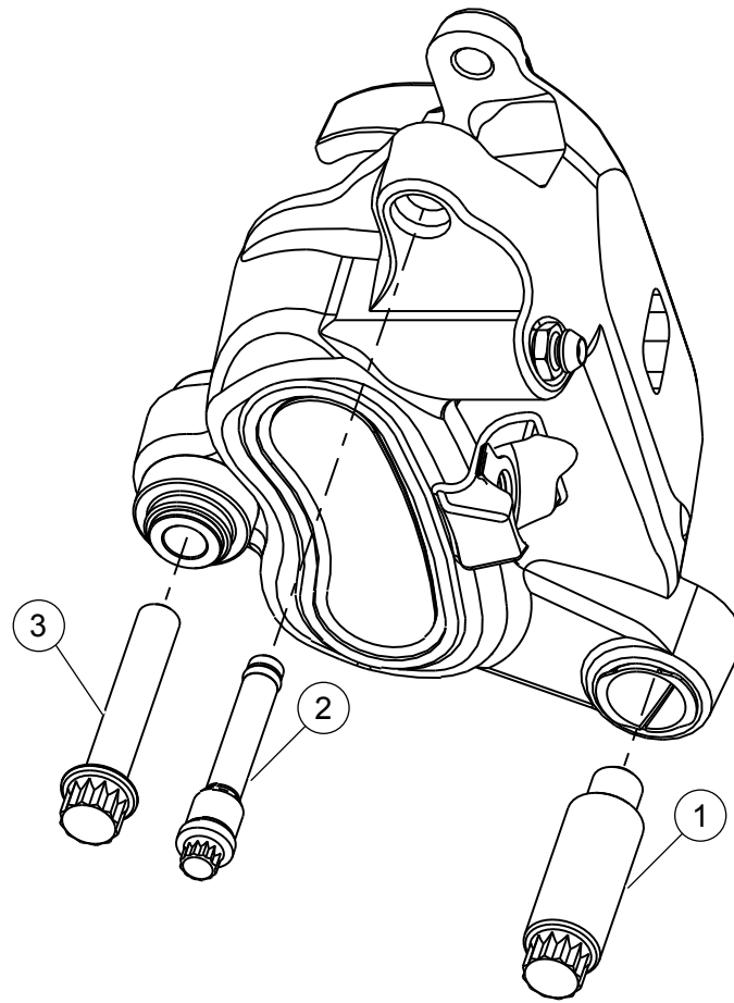
Figure 2. Service Parts: Chrome Brake Caliper Kit Mounting Hardware
