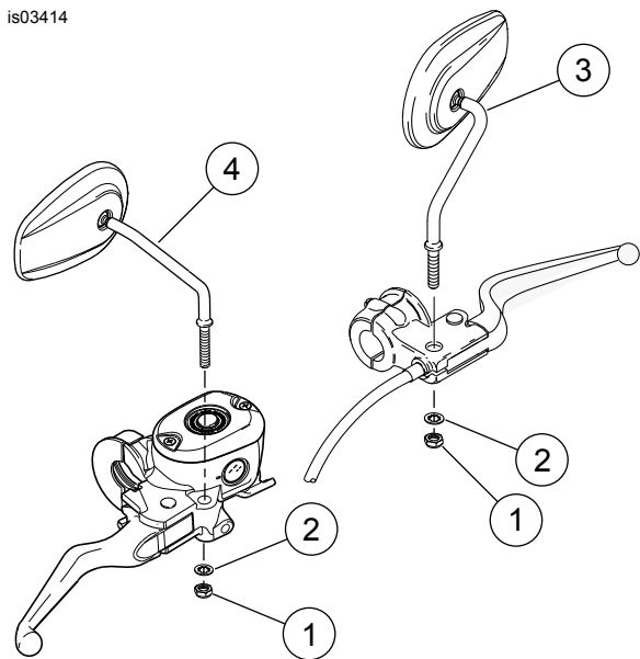
Figure 2. Remove Right Mirror (Touring, Softail - Except FXSTD, FLSTF)
