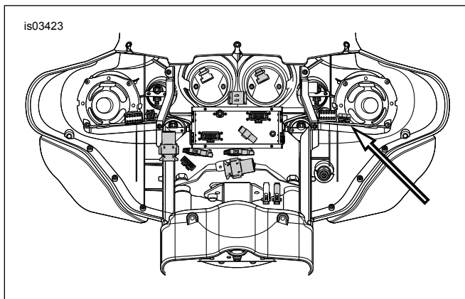
Figure 13. Front Turn Signal Connector (2005 and Earlier FLHT/C/U)
