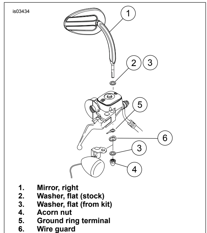
Figure 6. Install Right Lighted Mirror (Except Sportster, Dyna, FXSTD, FLSTF, FXSTS, FLSTS, VRSC)
