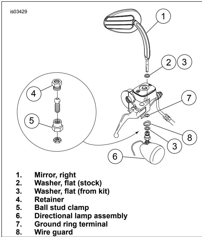
Figure 7. Install Right Lighted Mirror (Dyna, FXSTD, FLSTF, VRSC)
