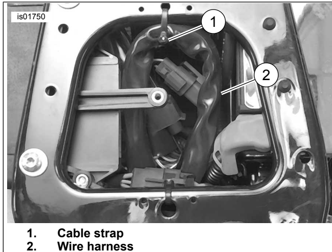
Figure 20. Dyna Service Loop (2005 and Earlier)
