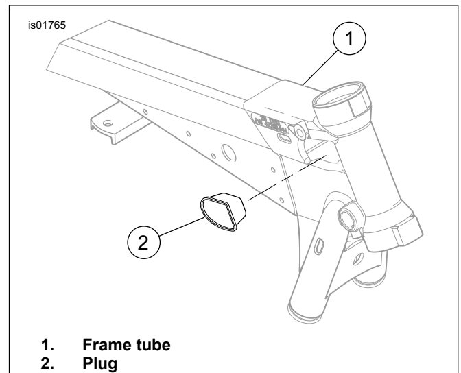
Figure 21. Dyna Top Frame Tube (2005 and Earlier)
