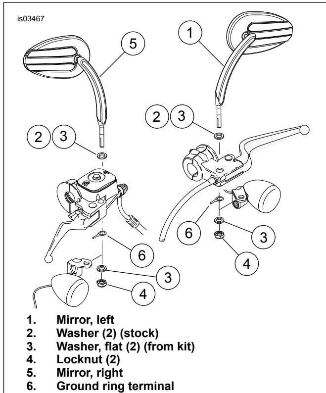
Figure 8. Install Lighted Mirrors (FXSTS, FLSTS)
