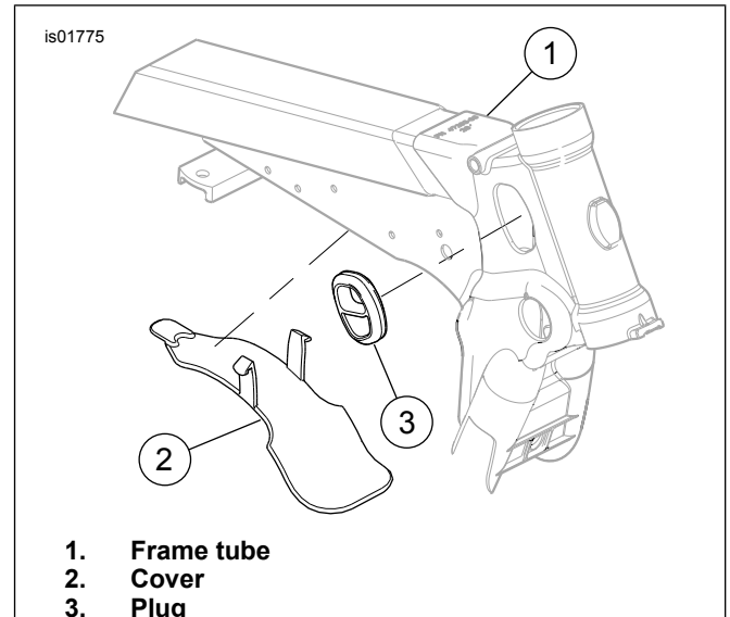
Figure 22. Dyna Top Frame Tube (2006 and Later)
