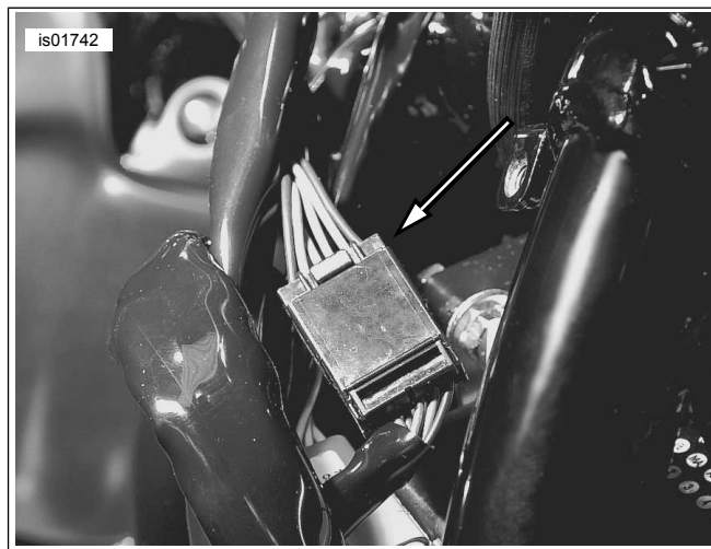
Figure 24. V-Rod Front Turn Signal Connector (2004 and Later)
