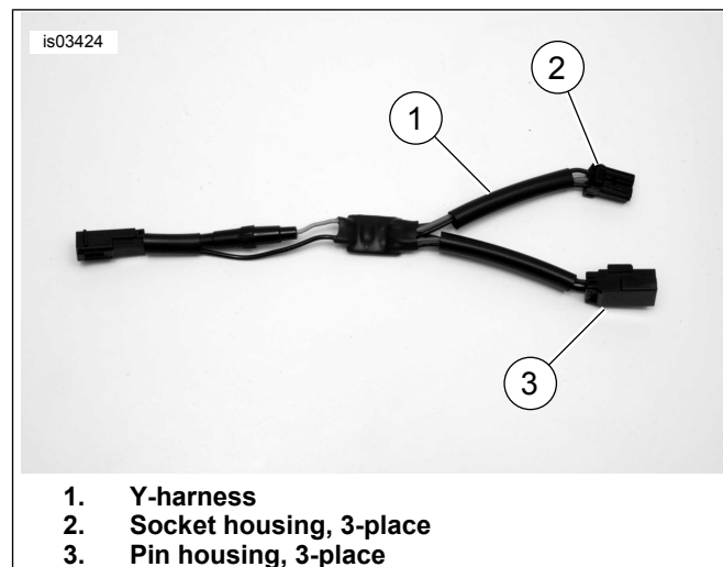
Figure 13. Front Turn Signal Connector (2005 and Earlier FLHT/C/U)
