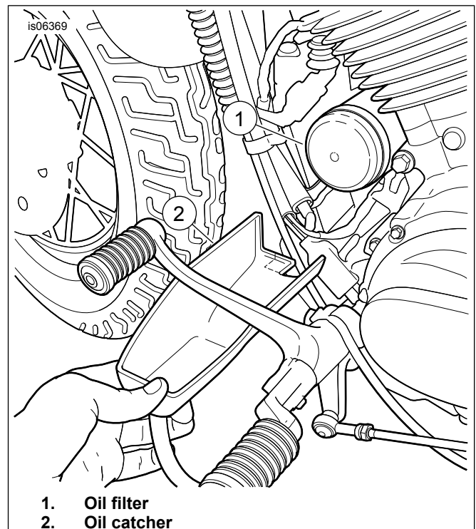
Figure 2. Oil Catcher
