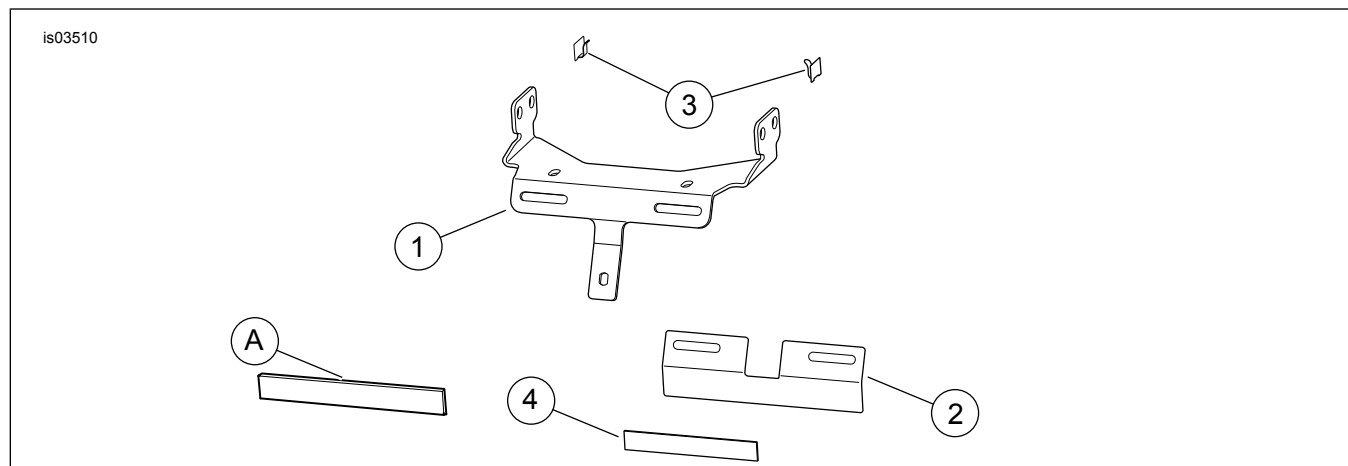
Figure 8. Service Parts Illustration: Bobtail Rack Support
