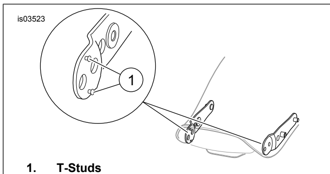
Figure 3. T-Stud Removal
