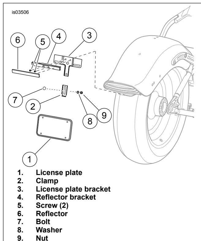
Figure 1. License Plate Bracket and Reflector Removal
