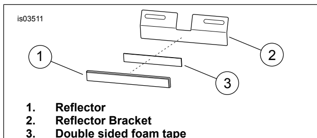
Figure 6. Attaching Reflector to Reflector Bracket
