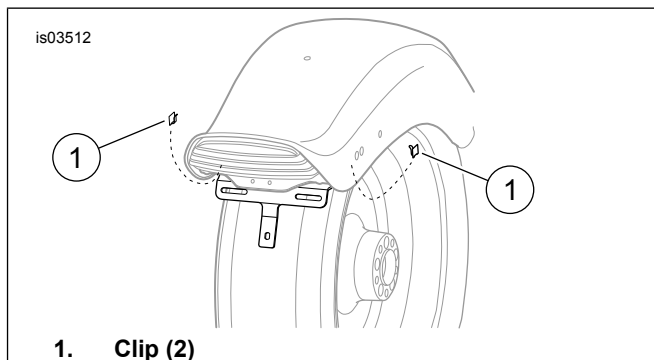
Figure 5. Clip Installation
