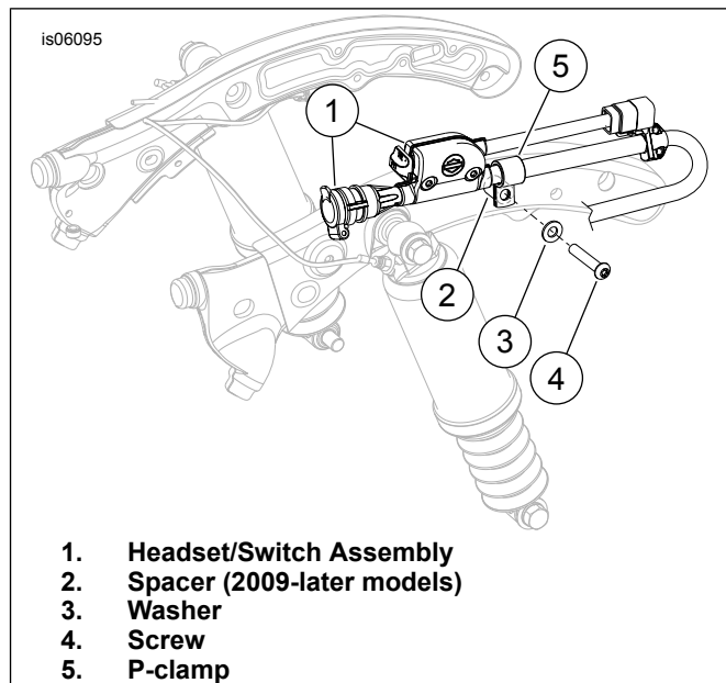
Figure 2. Installation Without Docking Points
