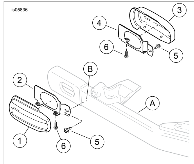
Figure 1. Service Parts, FXD Rear Axle Nut Cover Kit
