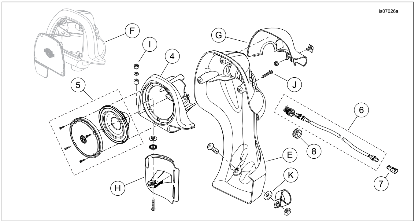
Figure 10. Service Parts, Custom Touring Audio System; Lower Fairing Speakers (See Table 2)
