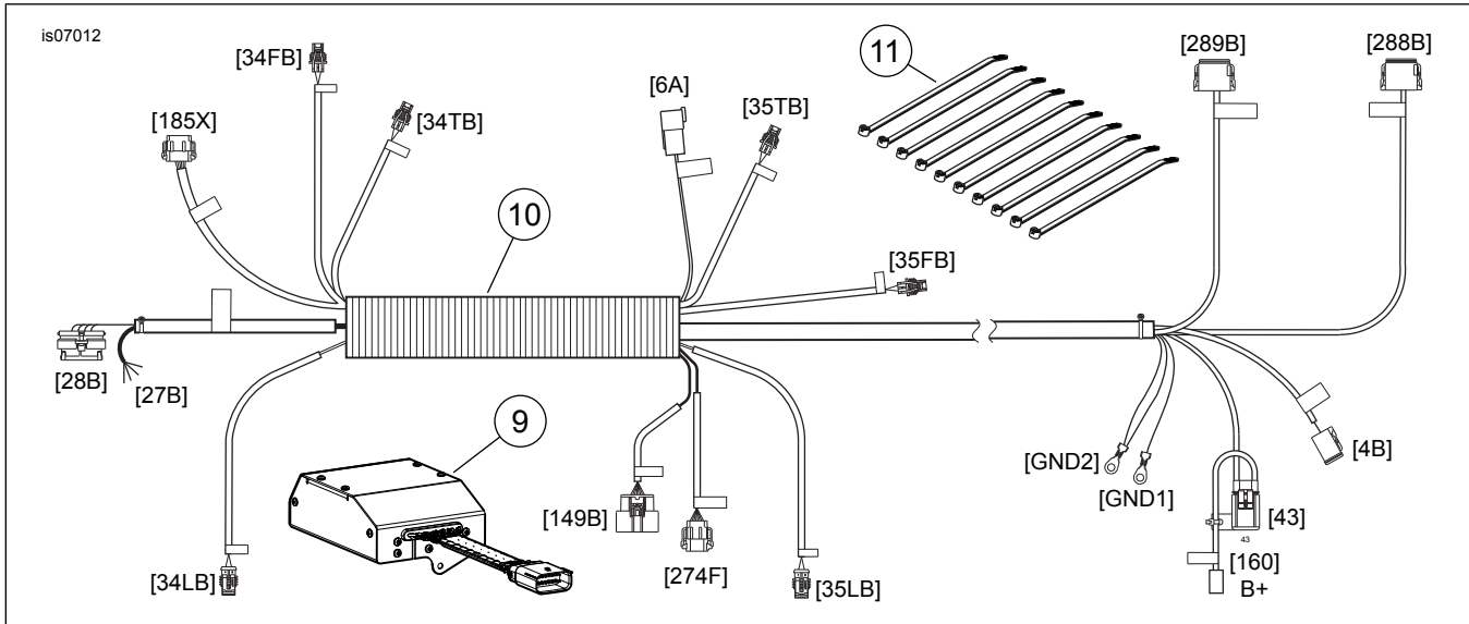
Figure 11. Service Parts, Custom Touring Audio System; Front Amplifier and Audio Harness (See Table 3)
