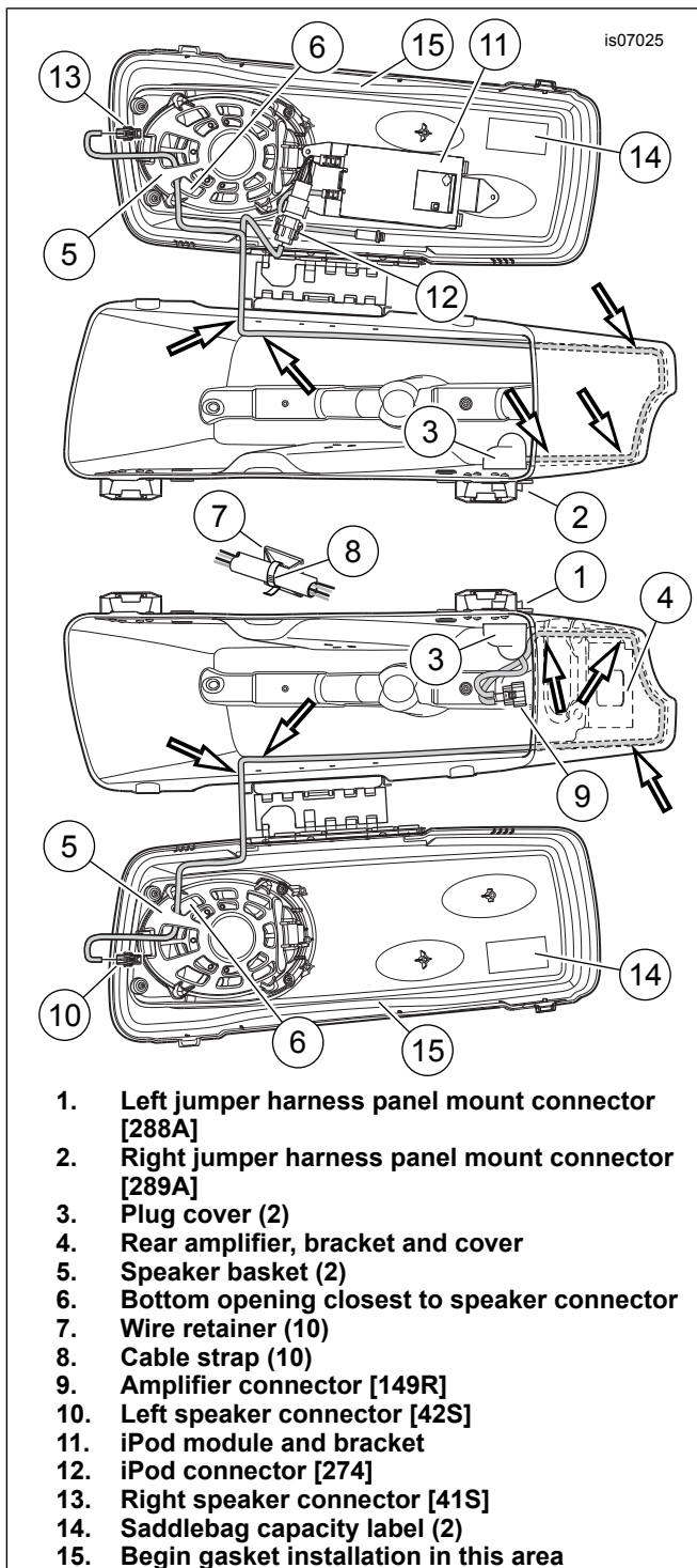
Figure 8. Harness Routing Inside Saddlebags
