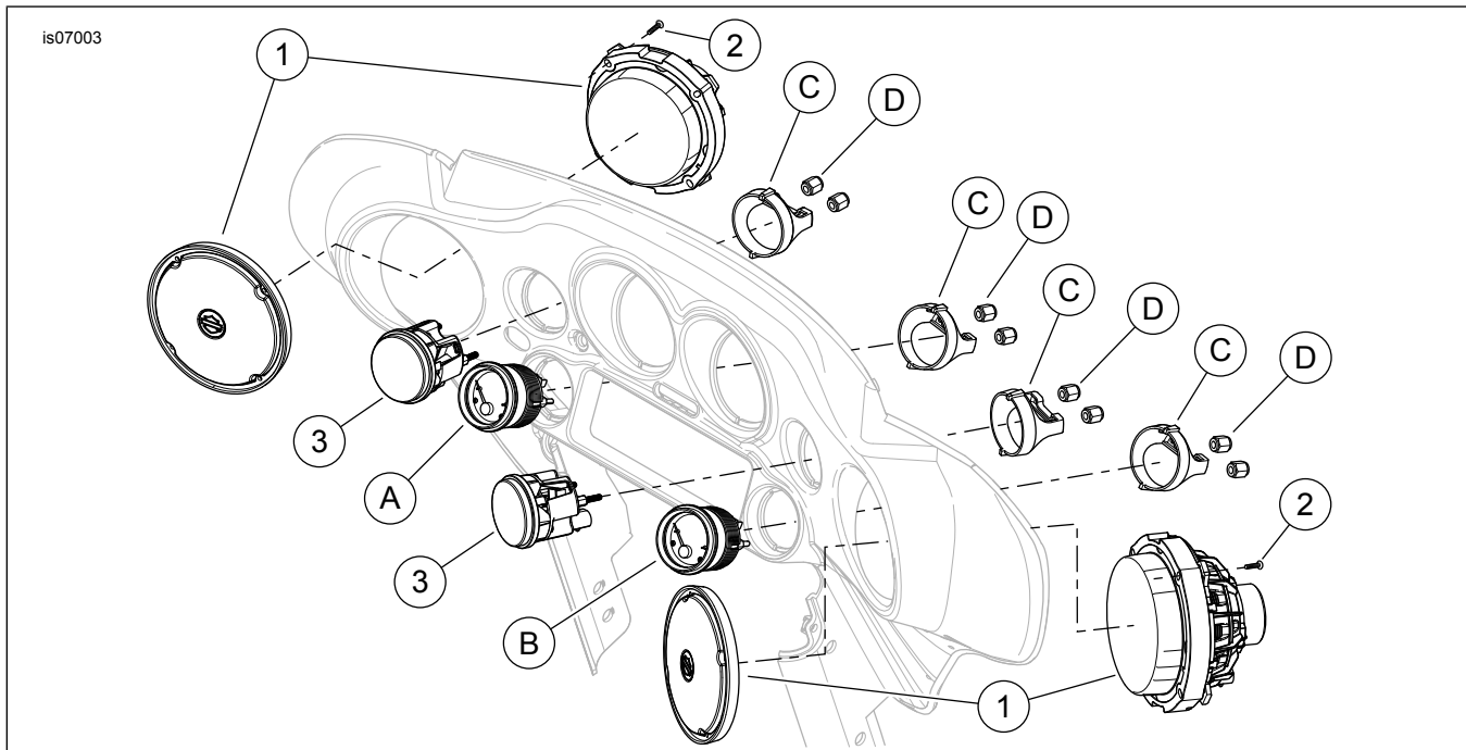
Figure 9. Service Parts, Custom Touring Audio System; Upper Fairing Speakers (See Table 2)
