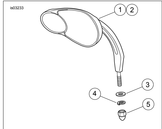
Figure 1. Service Parts: Split Vision Mirror
