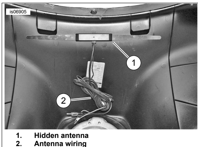
Figure 1. Electra Glide, Street Glide and Trike Installations
