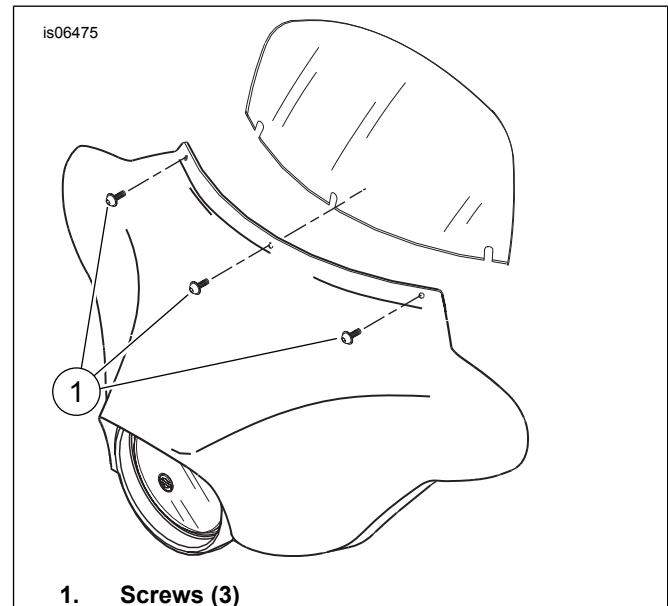
Figure 1. Fairing / Windshield Screws
