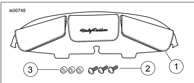
Figure 5. Service Parts: Fairing Pouch
