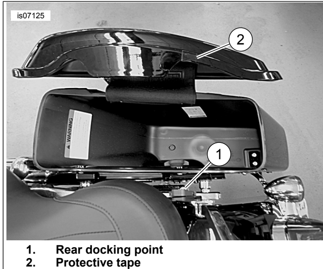
Figure 1. Installing Protective Tape
