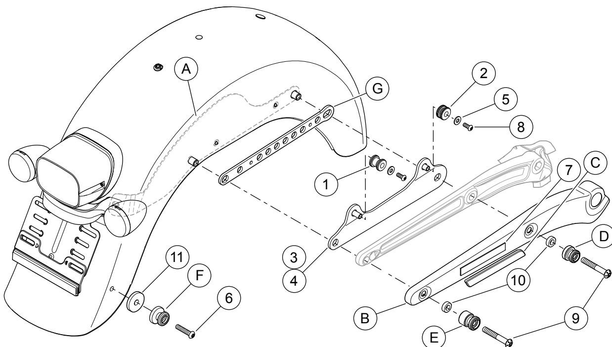
Figure 2. Service Parts: FLD Docking Hardware
