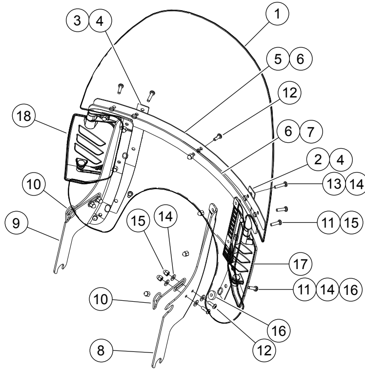
Figure 1. Service Parts: Vented Detachable Windshield
