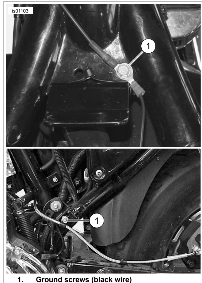
Figure 3. Ground Connections (Sportster Models)
