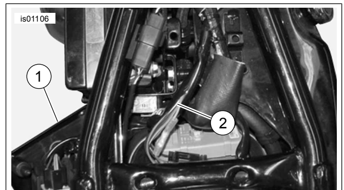
Figure 10. Power Connections (XL Models)
