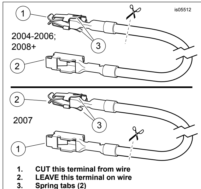
Figure 12. Fuse Block Adapter Wire (FL Touring)
