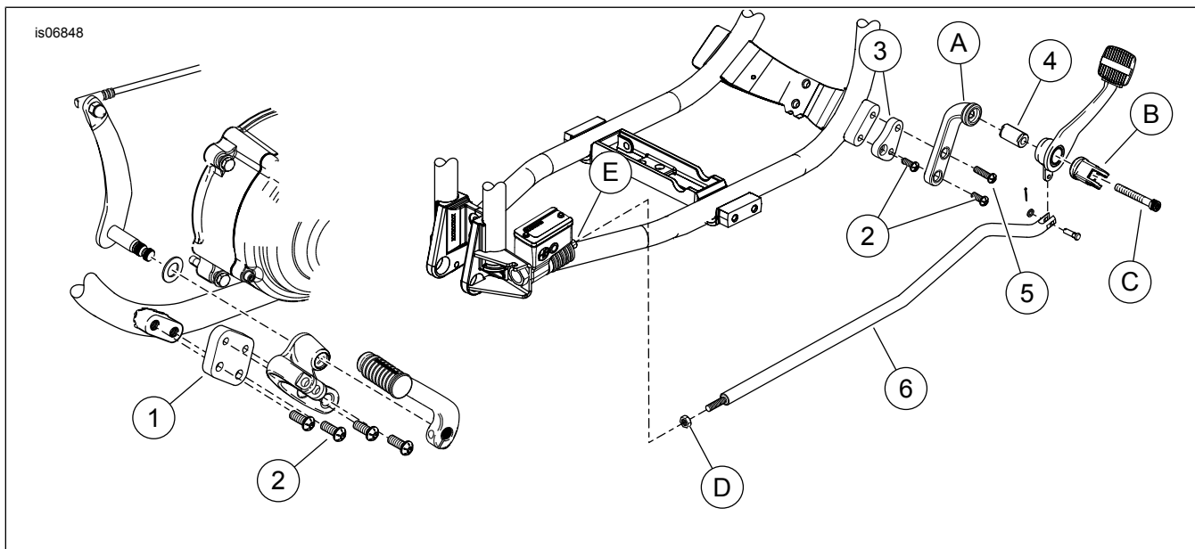
Figure 1. Service Parts: Reduced Reach Conversion Kit
