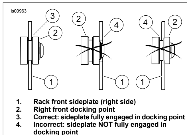
Figure 1. Luggage Rack Fit to Front Docking Points
