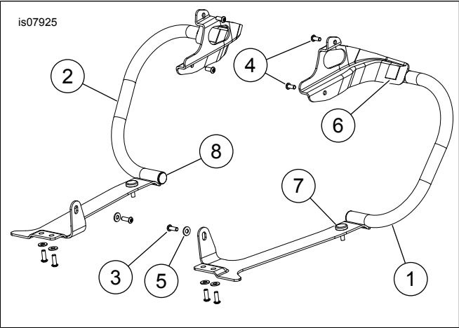
Figure 3. Service Parts: Saddlebag Guard Rail
