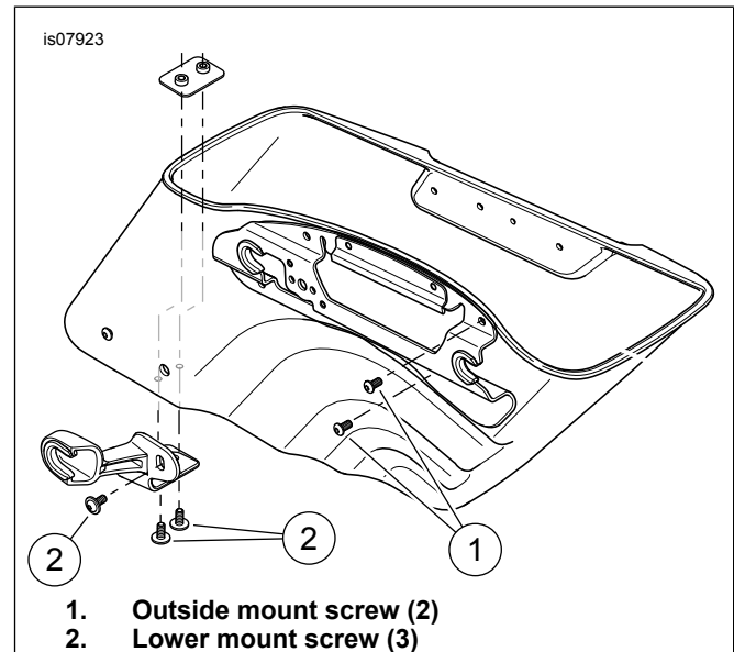
Figure 1. Saddlebag Screws
