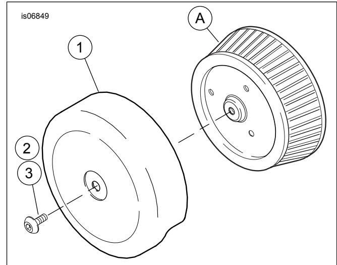
Figure 1. Service Parts: Air Cleaner Cover Kit
