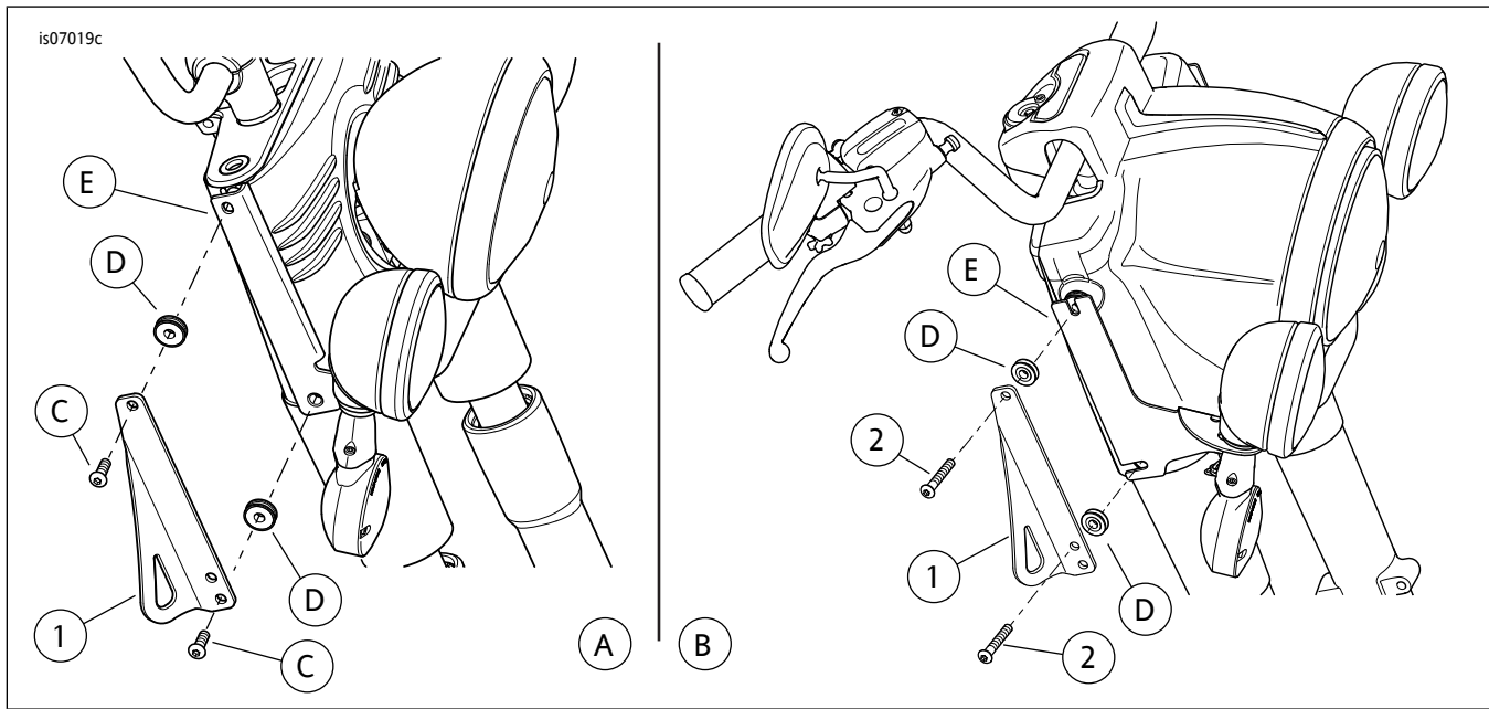
图1。安装捆绑带支架
