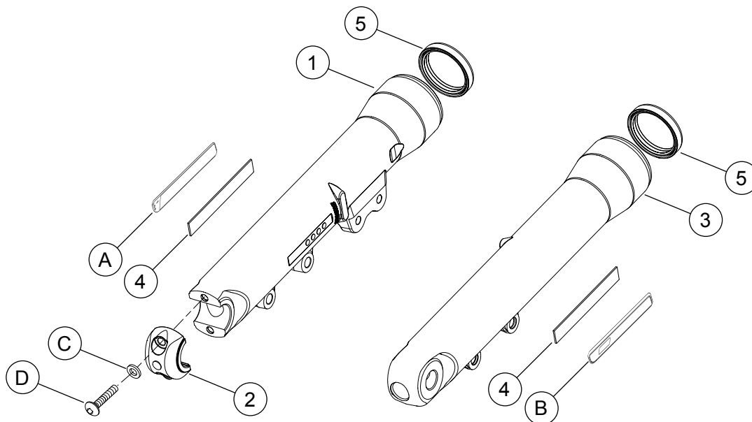
Figure 2. Service Parts: Dyna Fork Slider Kits
