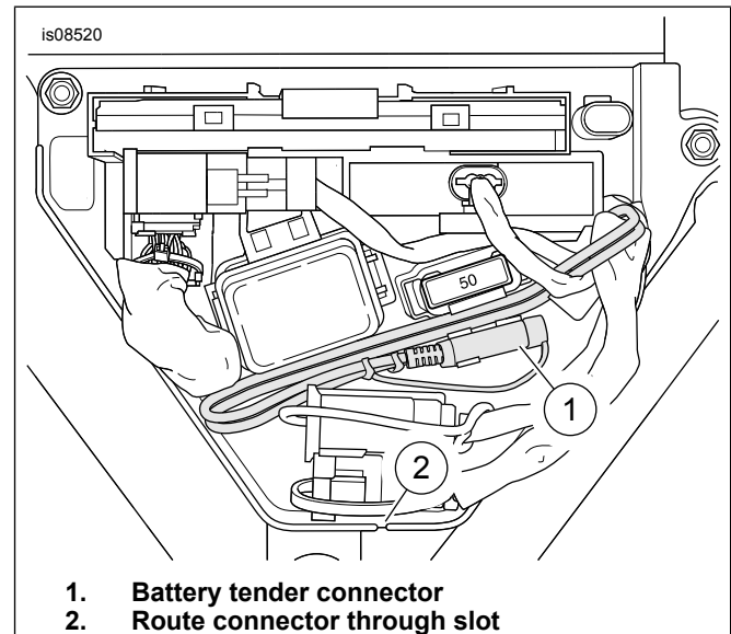
Figure 1. Battery Tender Connector
