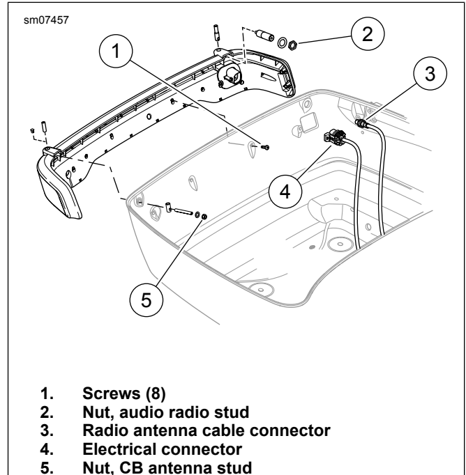
Figure 1. Wrap-around Lamp
