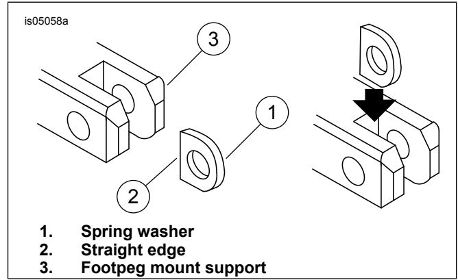
Figure 1. Vintage White Footpeg Spring Washer Installation
