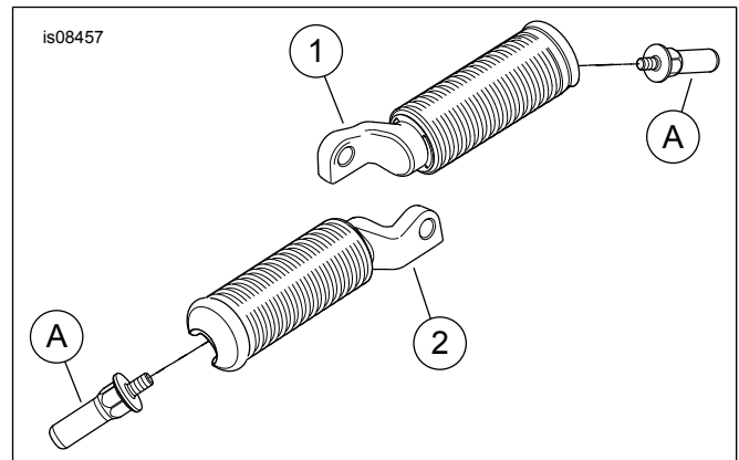
Figure 2. Service Parts: Vintage White Footpegs with Wear Pegs
