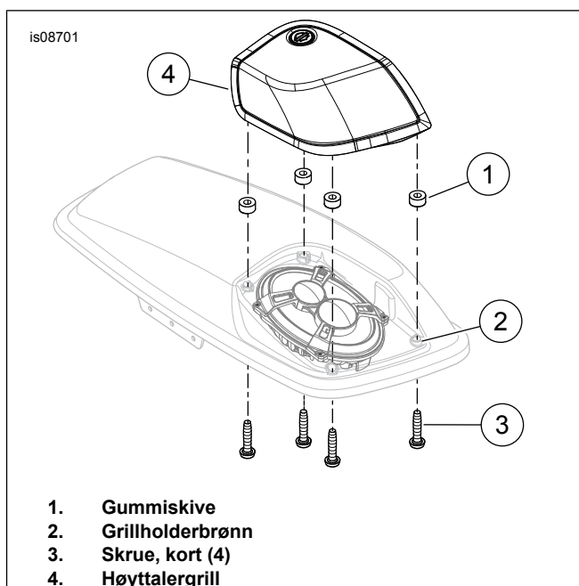
Figur 2. Grillmontering
