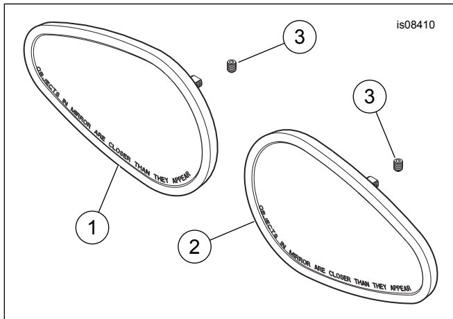
Figure 1. Service Parts, Windshield Trim Mirror Kit
