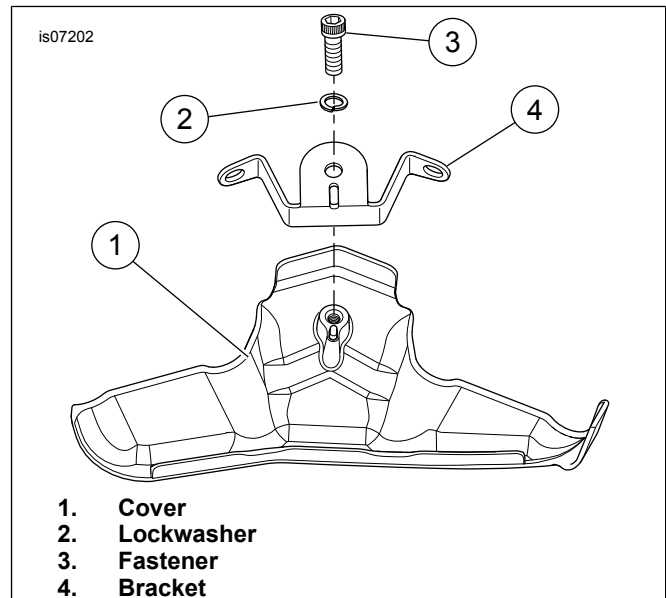
Figure 2. Bracket
