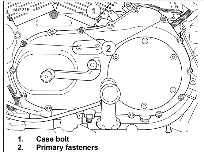
Figure 1. Remove Fasteners
