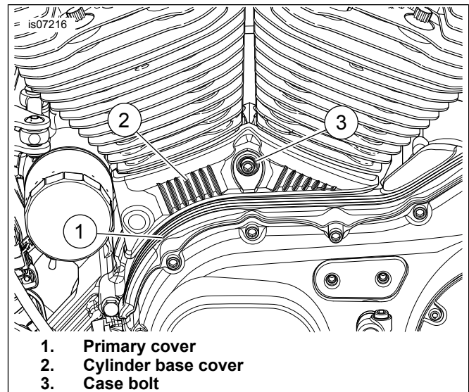
Figure 2. Primary And Cylinder Base Covers
