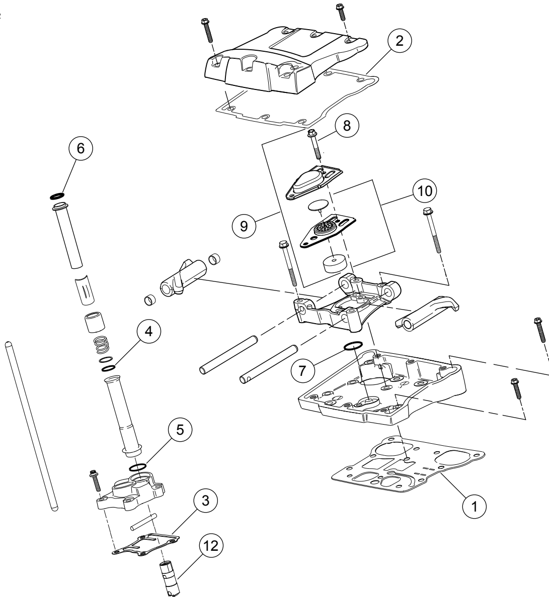
Figure 2. Service Parts: Screamin' Eagle Twin Cam 110 (1800 cc) Bolt-on Conversion Kit
