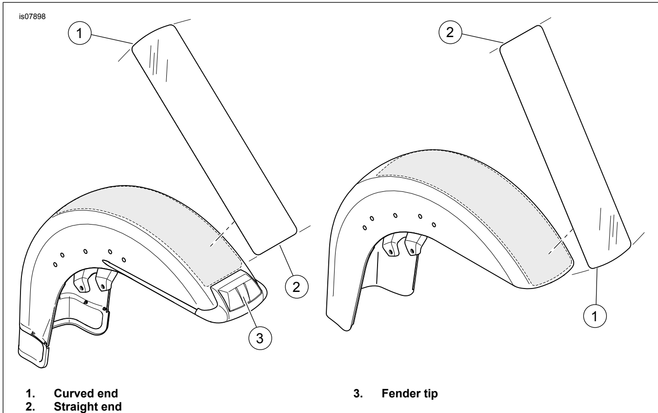
Figure 1. Tape Orientation
