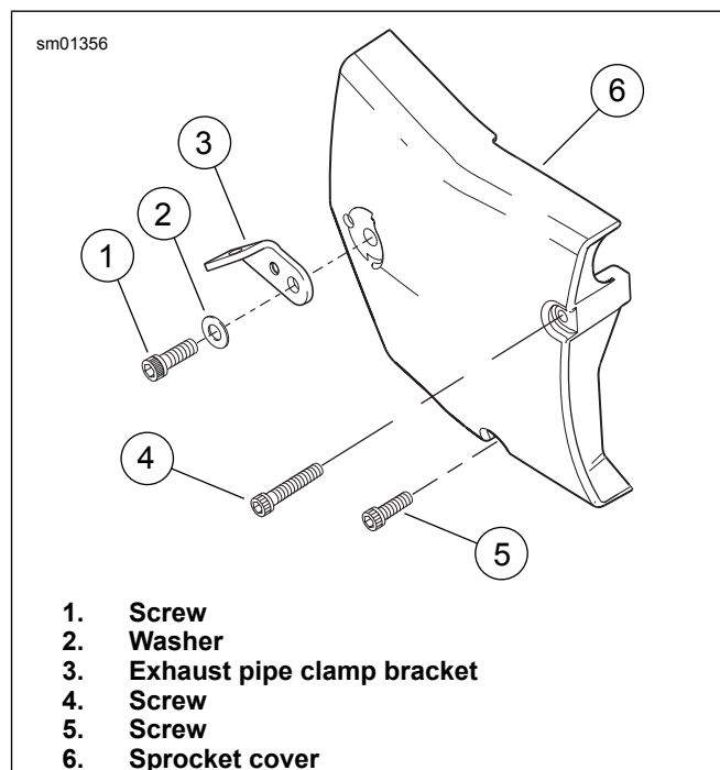
Figure 1. Sprocket Cover
