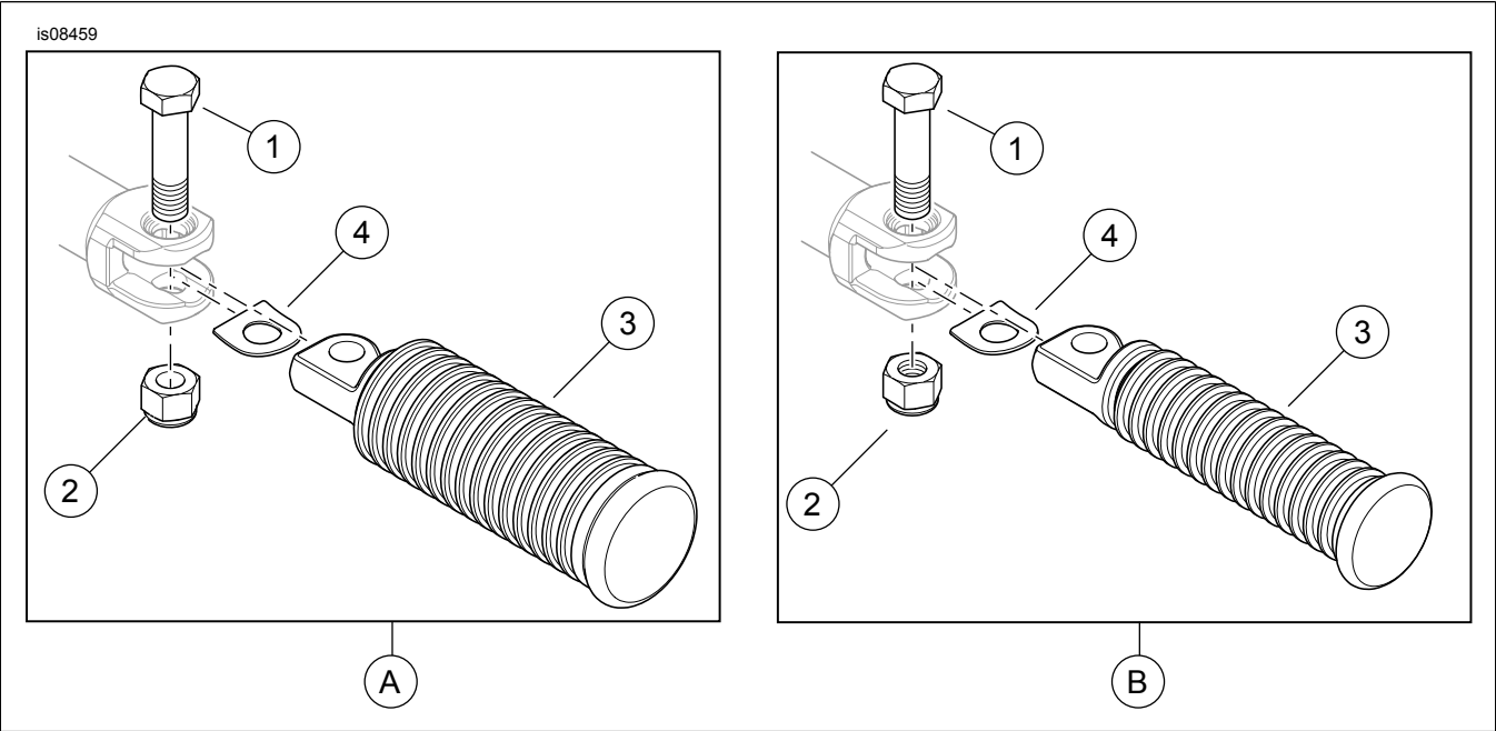
Figure 2. Service Parts: Footpegs
