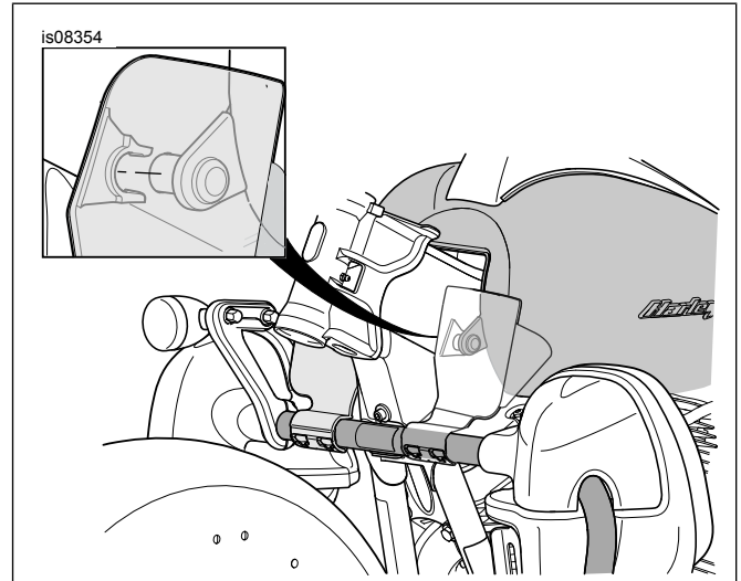
Figure 1. Air Deflector
