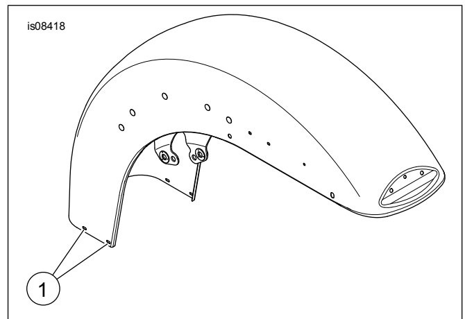
Figure 1. Clean Front Fender Hole Locations
