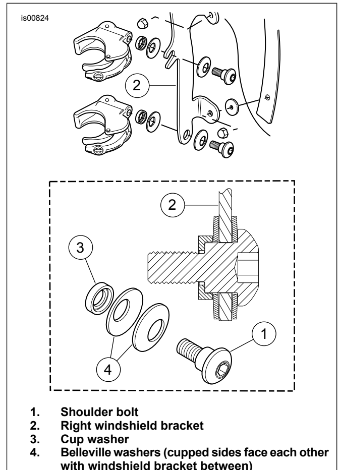
Figure 1. Windshield Mounting Clamp
