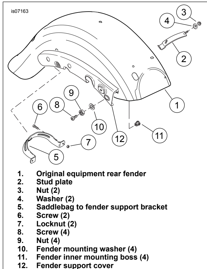
Figure 2. Remove Rear Fender Items
