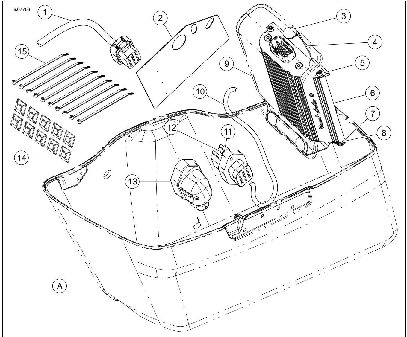
Figure 14. Service Parts, Boom! Audio Amplifier Expansion Kit
