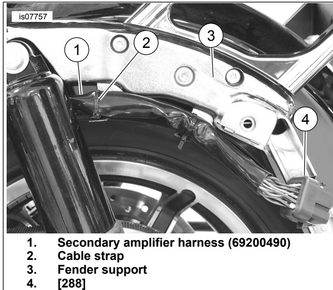
Figure 12. Harness Routing
