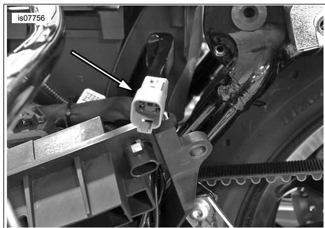
Figure 11. DLC [91A]
