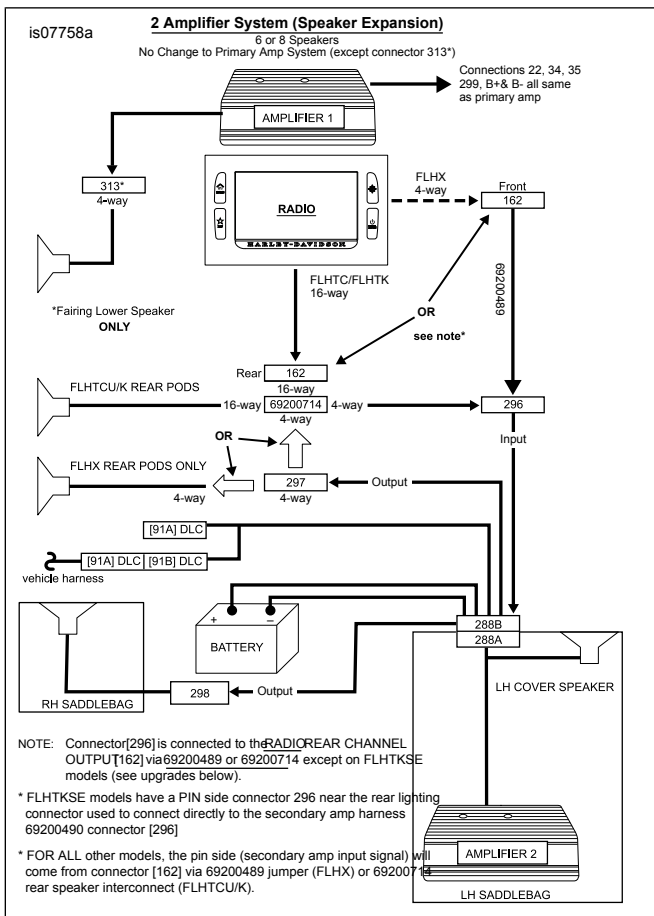
Figure 13. Amplifier System
