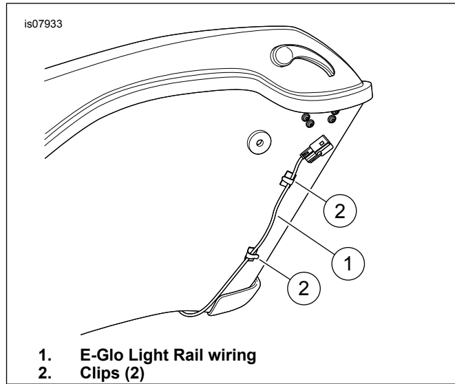
Figure 2. Wire Routing
