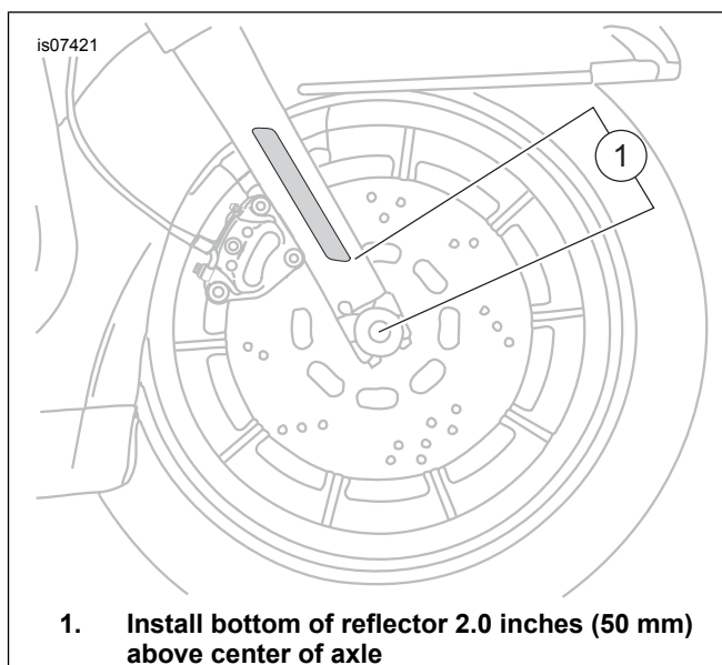
Figure 1. Reflector Placement
